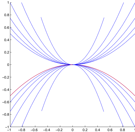
FIGURE 4. Our approach showing focusing on an initial inverted parabola. A singularity forms at the critical time but before and afterwards, the solution is not multi-valued.
