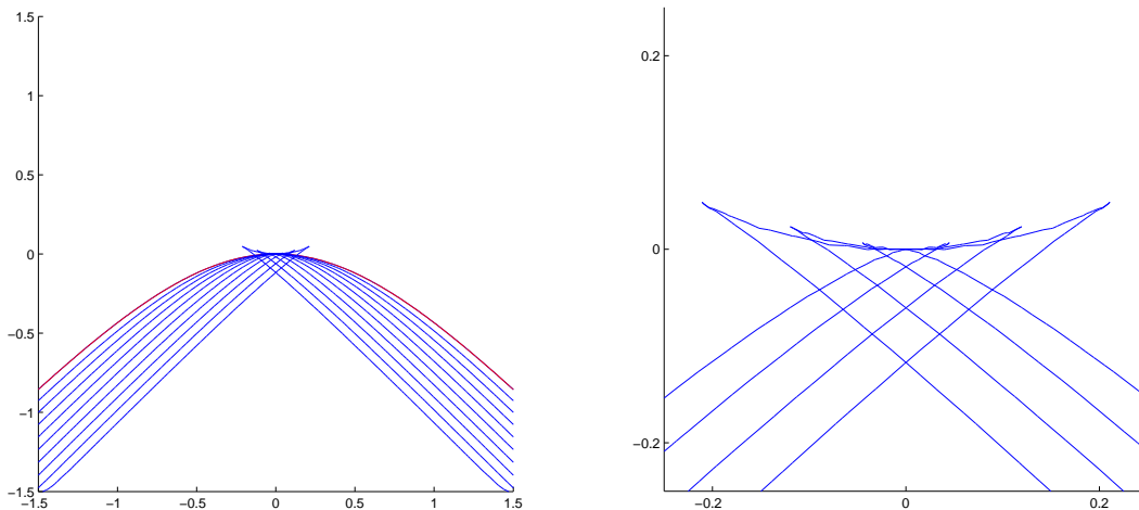
FIGURE 5. Our approach capturing caustics, with a swallow-tail multi-valuedness developing at the critical time. The figure on the right is a zoomed picture around the singularity of the solutions at and after the critical time.
