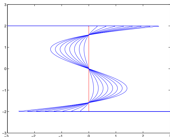
FIGURE 2. Our approach applied to a Riemann problem that produces multi-valued solutions.
