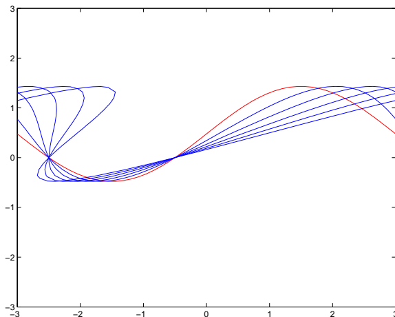
FIGURE 1. Our approach capturing a sine function overturning to become multi-valued.
