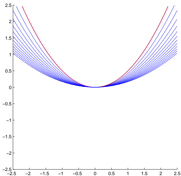
FIGURE 3. Our approach for free motion on an initial parabola. No singularities appear in this example.
