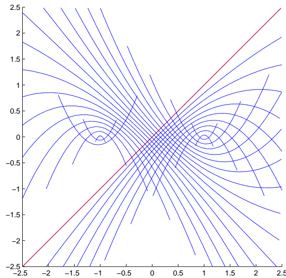
FIGURE 6. Our approach for the harmonic oscillator showing oscillating focusing effects occurring between two points.
